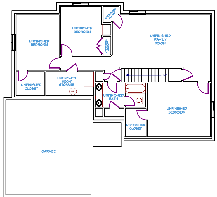
FOUNDATION PLAN
